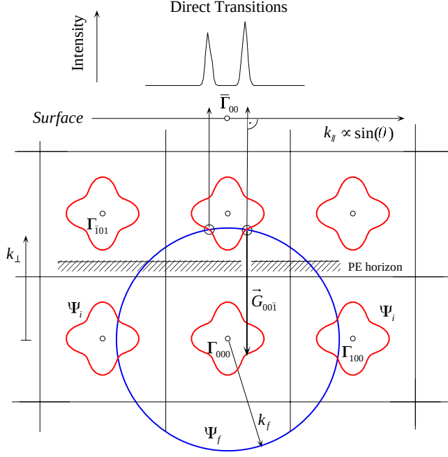
Fig. 4. Photoemission process for band mapping in a k_{\parallel} vs. k_{\perp} picture. Wherever the final state band \Psi_f crosses an initial state band of the periodic zone scheme \Psi_i a direct transition occurs. This transition may be observed above the photoemission (PE) horizon that is a consequence of the surface barrier potential.
