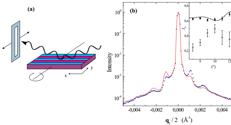
Fig. 2. (a) Experimental geometry with x-rays incident along the stripe direction at grazing angle, \Theta . Scattered x-rays were detected by a photodiode mounted behind a rectangular aperture. (b) Diffraction scans with the wavevector, \mathbf{q}_y transferred along the y -axis. Left-circularly polarized (dotted line, I^- ) and right-circularly polarized (solid line, I^+ ) x-rays with energy tuned to the Fe L_3 absorption edge impinge at an angle of \Theta = 12^\circ relative to the surface plane. The inset shows the values of I_A = (I^+ - I^-)/(I^+ + I^-) for first-order (solid symbols) and second-order (open symbols) magnetic satellite peaks. [27]
