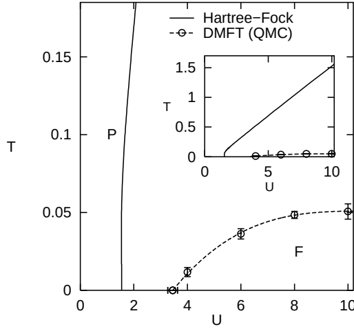
Fig. 5. T vs. U phase diagram for a strongly peaked DOS ( a = 0.98 , see Fig. 4b) at n = 0.4 within DMFT (circles; dashed line is guide to the eyes only) in comparison with Hartree-Fock (solid line) [38].
