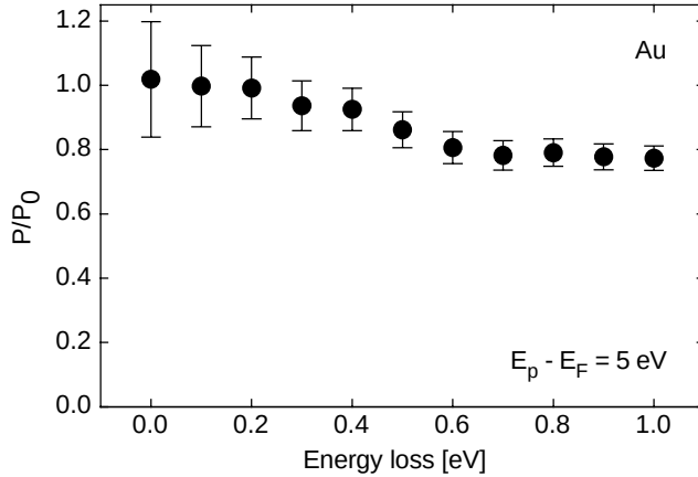
Fig. 3. The degree of relative spin polarization P/P_0 after the electron beam has traversed a pure Au-film is shown as a function of energy loss. P_0 is the degree of spin polarization delivered by the electron source. The primary energy E_p of the incident electron beam is 5 eV above the Fermi energy E_F
