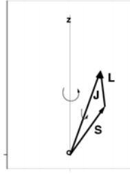
Fig. 1. LS-coupling of Angular momenta J , L and S . A small magnetic field, B , is pointing along the k -direction (from o to z ).
