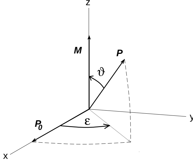
Fig. 1. Schematic drawing of the two types of movement of the spin polarization vector for |\mathbf{P}_0| = 1 (pure spin state). Due to the difference in the amplitude of the majority-spin and the minority-spin wave function, the spin polarization vector rotates towards the sample magnetization \mathbf{M} , i.e., the angle \vartheta decreases. The difference in the phase factors, on the other hand, causes the spin polarization vector to precess around \mathbf{M} by an angle of \epsilon
