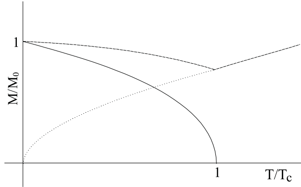
Fig. 3. Temperature dependence of the bulk moment \sqrt{\left(1 - \frac{T}{T_c}\right)} (full curve), the fluctuations \sqrt{\frac{3}{5} \frac{T}{T_c}} (dotted curve), and the order parameter \sqrt{\left(1 - \frac{2}{5} \frac{T}{T_c}\right)} (dashed curve).
