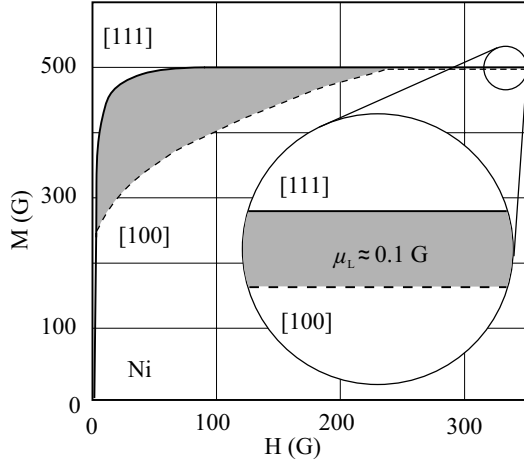
Fig. 1. Room temperature magnetization curve for Ni along the easy ([111]) and hard ([100]) direction [17]
