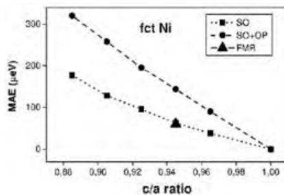
Fig. 8. Calculated and measured (filled triangle) values of the MAE (in plane minus out-of-plane) of bulk fct Ni. The calculations were made as a function of c/a ratio, with and without the orbital polarization correction. Positive numbers indicate the 001 direction as the easy axis.
