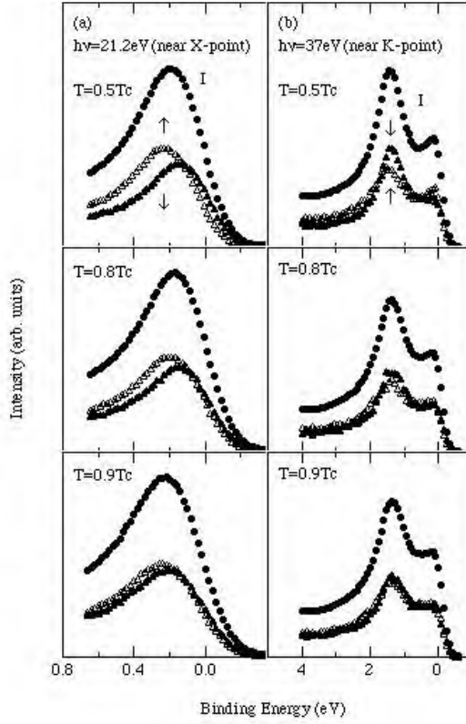
Fig. 6. Temperature dependence of the spin-resolved photoemission spectra of Ni(110) near (a) X -point and (b) K -point in the B.z. Spin integrated spectra (I) are sum of majority ( \triangle ) and minority ( \blacktriangle ) spin spectra. In both figures, majority and minority spin spectra show collapsing behavior as temperature approaches to T_c .
