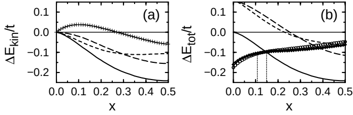
Fig. 6. Energy gain for various phases with respect to the FO state with complex orbitals (18) versus hole doping x : (a) kinetic energy \Delta E_{\text{kin}}/t , and (b) total energy \Delta E_{\text{tot}}/t . Here |\Phi_x\rangle , |\Phi_z\rangle (9), AO state with complex orbitals (18), and OL state, are shown by dashed lines, long-dashed lines, pluses, and full lines, respectively. The AO states with A-AF (circles) and FI (diamonds) order [part (b)] are more stable than the OL state at low doping x ; two phase transitions are indicated by vertical dotted lines.
