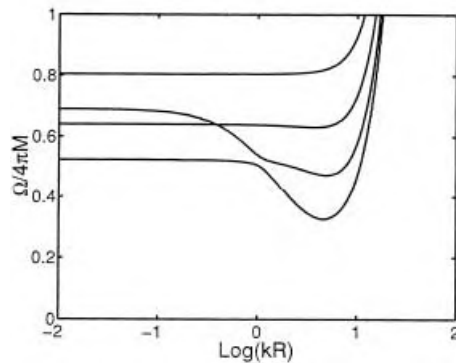
Fig. 2. For m = 1 , h = .19 and p = .05 , we show the spin wave frequencies of the nanowire plotted as a function of \log(kR) .
