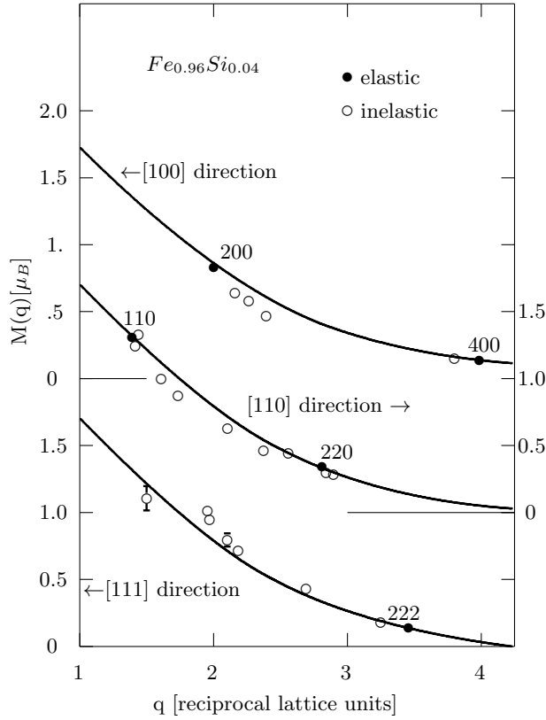
Fig. 1. Fourier transform of the magnetisation density M(\mathbf{q}) for bcc iron as measured on a phonon (hollow circles) and compared to the static magnetisation density (smooth curve) as measured on Bragg reflections. Full circles indicate an elastic measurement carried out on a Bragg reflection. Data taken from Steinsvoll et al. [10].
