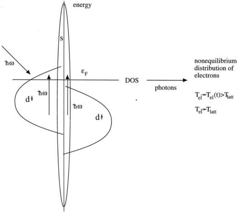
Fig. 1. Illustration of the scenario for the non-equilibrium state produced by exciting optically electrons out of the ground state (the Fermi sea). \epsilon_F is the Fermi-energy. The hot electrons relax first due to electron-electron interactions. The electron thermalization is characterized by the electron temperature T_{el}(t) . Energy transfer from the electrons to the lattice occurs via the electron-lattice coupling and which controls T_{el}(t) for longer times. Time resolved spectroscopy observes the dynamics of the hot electron distribution n(t) . A spin split density of states N(E) or circularly polarized light creates a spin-polarization of the hot electrons
