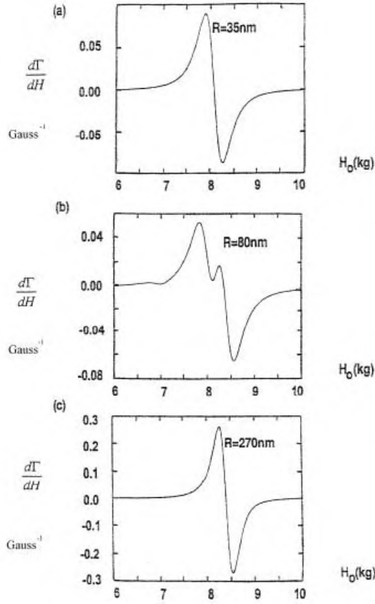
Fig. 6. For three values of the radius of Ni nanowires, (a) 350 Angstroms, (b) 800 Angstroms, and (c) 2700 Angstroms, we show calculated ferromagnetic resonance spectra. The calculations employ G = 2.5 \times 10^8 \text{ sec}^{-1} which is a realistic value for Ni, and we have taken K_S = -0.85 \text{ ergs/cm}^2 .
