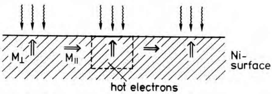
Fig. 5. Light induced magnetic pattern at surfaces due to magnetic reorientation M_{\perp} \rightarrow M_{\parallel} in response to hot electrons, T_{el}(t) . Note, the response time for the reorientation transition is given by t_R \sim E_{anisot} \sim 100ps in transition metals, for example
