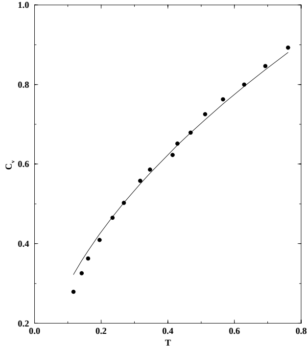
Fig. 3. Plot of C_v as a function of T for CeCu_{5.7}Au_{0.3} at a pressure of 8.2 kbar. The experimental points [20] are represented by circles and the solid line represents the theoretical fit (from [10]).
