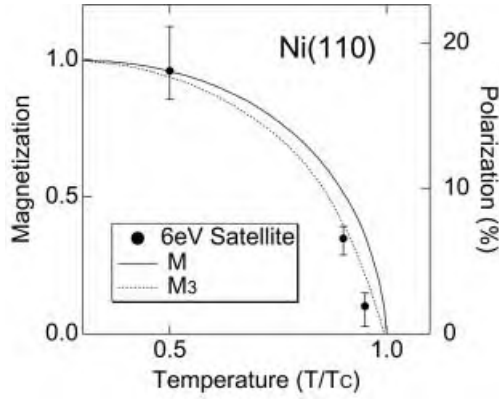
Fig. 9. Temperature dependence of the characteristic spin polarization of the 6 eV satellite. The solid and dotted curves represent the temperature dependence the macroscopic magnetization and the magnetization of 3 ML in the mean field theory, respectively. Experimental results are normalized to the macroscopic magnetization at T/T_c = 0.5 .
