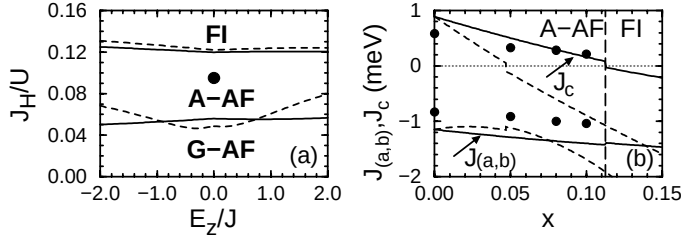
Fig. 1. (a) Mean-field phase diagram of \text{LaMnO}_3 obtained using SE interactions H_J^e and H_J^t (dashed lines), and both SE and cooperative JT effect H_{\text{JT}} (full lines); the parameters of \text{LaMnO}_3 [19] are indicated by a dot. (b) Exchange interactions J_{(a,b)} and J_c as functions of doping x for the states with OO (full lines), and for orbital polarons (dashed lines), compared with experimental data for \text{La}_{1-x}\text{Ca}_x\text{MnO}_3 (dots) [21].
