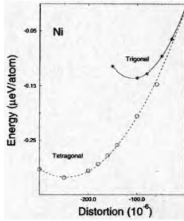
Fig. 10. Calculated magnetostriction \lambda_{111} and \lambda_{001} for Ni, using the total energy approach (circles and asterisks) and Eqn.2 (full and dashed lines).
