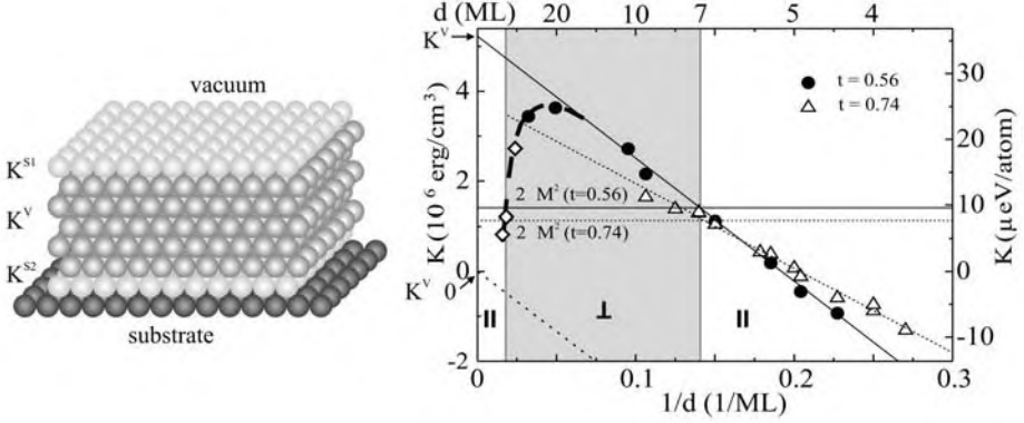
Fig. 4. Left panel: Schematic drawing of a pseudomorphic grown thin film with 3 contributions of anisotropy energy contributions, the surface term K^{S1} , the interface term K^{S2} and the central or volume term K^V . Right hand panel: Experimental data for Ni/Cu(001) taken from [28]. If, hypothetically, the Ni film would grow in a pseudomorphic structure up to infinite thickness ( 1/d = 0 ), K^V would reach a value indicated on the y -axis. This is by orders of magnitude larger than for unperturbed bulk fcc Ni as indicated close to the '0' of the y -axis. The 3 regimes indicate parallel, perpendicular and again parallel easy axis of magnetization. For details of the spin reorientation transition see [28,30].
