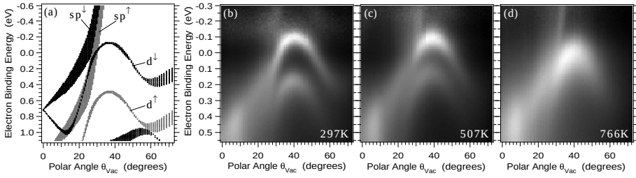
Fig. 7. (a) Spin-polarized LKKR calculation covering the section in \mathbf{k} -space of the measurements. Majority spin bands are given in gray, minority bands in black. (b)–(d): He I \alpha excited polar-angle scanned electron distribution curves EDCs taken from Ni(111) along the azimuth which is clock wise 23^\circ off [\bar{1}\bar{1}2] , measured at three different temperatures: (b) 0.47 T_C , (c) 0.80 T_C , and (d) 1.21 T_C . From Ref.[20].
