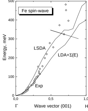
Fig. 5. The spin-wave spectrum for ferromagnetic iron in the LSDA and LDA+ \Sigma approximations compared with different experiments (circles [16], squares [17], and diamonds [18]) (a); The corresponding spin-wave spectrum from LDA+ \Sigma scheme in the (110) plane (b).
