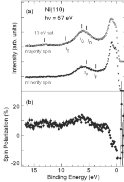
Fig. 7. (a) shows majority ( \Delta ) and minority ( \blacktriangle ) spin spectra of Ni(110) observed at the 3d threshold (67 eV). Vertical bars correspond to the positions of the 3d^8 final state configurations expected by an atomic model. (b) shows the spin polarization of Ni valence band. The statistical error is indicated by bars.
