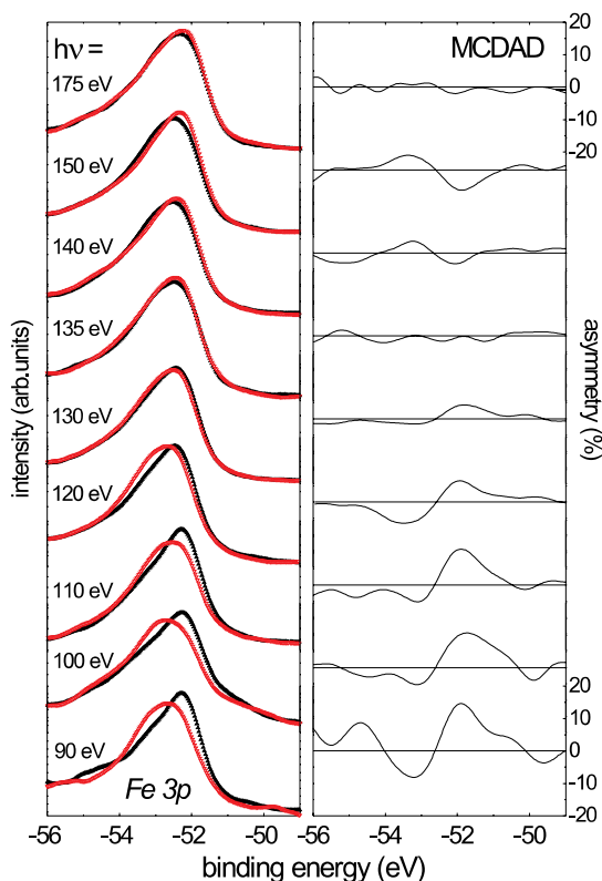
Fig. 4. Series of normal emission photoelectron spectra from the Fe 3p levels with Shirley background subtraction. The data have been taken with right circularly polarized radiation in the range between 90eV and 175eV, full and open triangles denote opposite magnetization states (left side). The full curves display the asymmetry results from a simple fitting procedure in order to guide the eye (right side).
