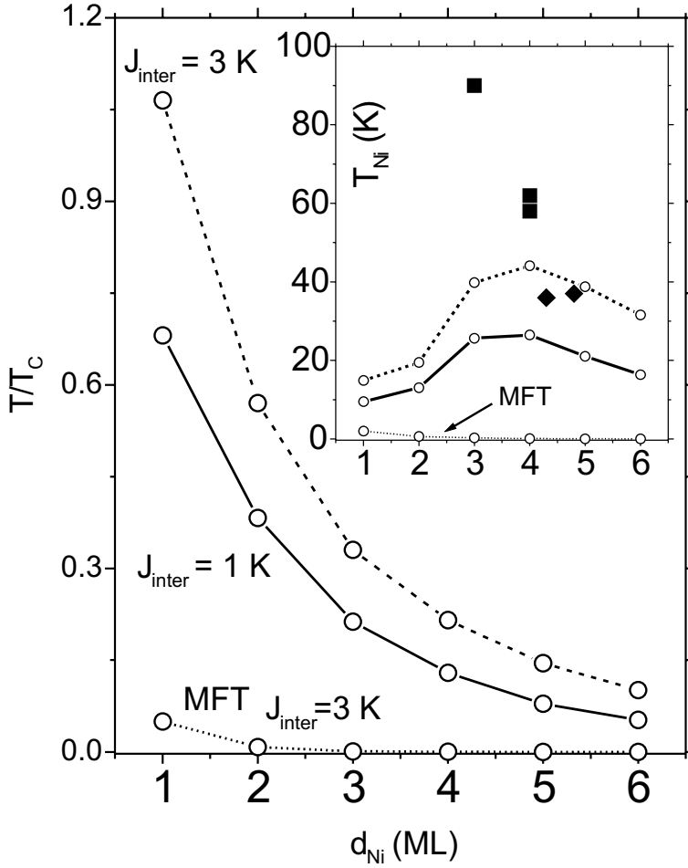
Fig. 5. Coupling-induced increase \Delta T_{\text{Ni}} , plotted in a reduced temperature scale, as a function of the number of Ni layers with J_{\text{inter}} as a parameter. In the inset calculations are compared to experimental data points. The calculations based on a mean-field theory (MFT) can not describe properly the experiment [36]. In other words, these experiments can not be realized in the bulk, but only in 2D magnets.
