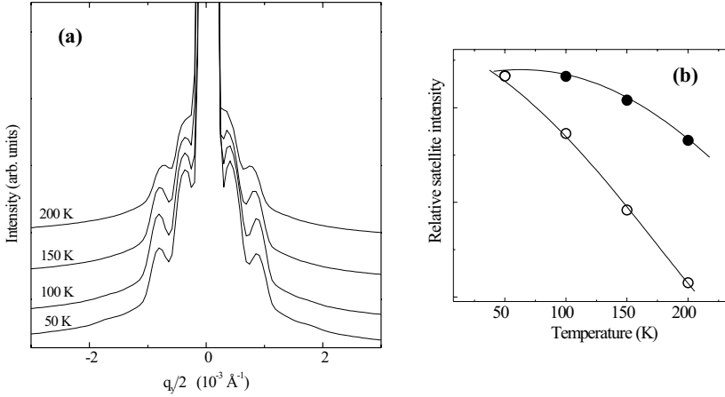
Fig. 3. (a) Fe L_3 -edge XRD scans from a Fe(16Å)/CeH 2 (10Å) multilayer measured at the indicated temperatures. (b) Temperature dependence of the normalized and background corrected intensity of the first-order (open circles) and second-order (solid circles) magnetic peaks of the spectra shown in (a) [34]. The lines serve as guides to the eye
