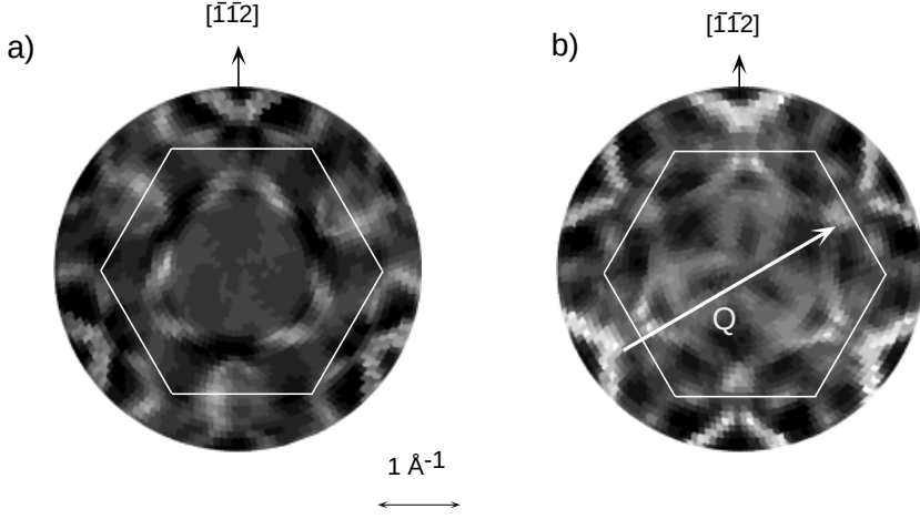
Fig. 8. Fermi surface map from a) Ni(111) measured with He I \beta radiation ( k_{\parallel} \leq 2.15 \text{ \AA}^{-1} ) and b) h -BN/Ni(111) measured with He I \alpha radiation ( k_{\parallel} \leq 2.15 \text{ \AA}^{-1} ) are shown. The differences of a) relative to the Fermi surface maps in Fig.5 are mainly given due to the normalization of the data of each azimuthal scan and much less due to the slightly different photon energy. The hexagons indicate the first surface Brillouin zone. The vector \mathbf{Q} indicates an umklapp process and is a reciprocal vector of the surface lattice. From Ref.[30].
