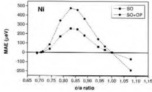
Fig. 9. Calculated values of the MAE (in plane minus out-of-plane) of bulk fct Ni. The calculations were made as a function of c/a ratio along the Bain path. Positive numbers indicate the 001 direction as the easy axis.
