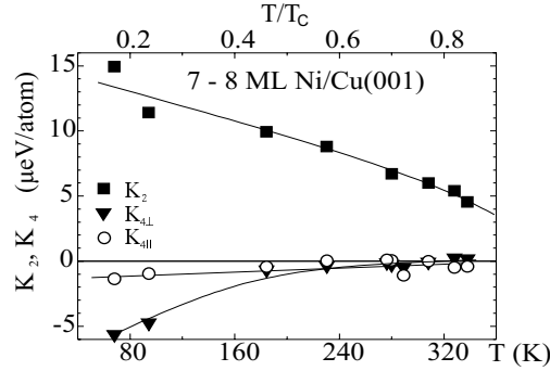
Fig. 8. Temperature dependence of K_2 , K_{4\perp} and K_{4||} for \approx 7.5 ML Ni/Cu(001) [38].
