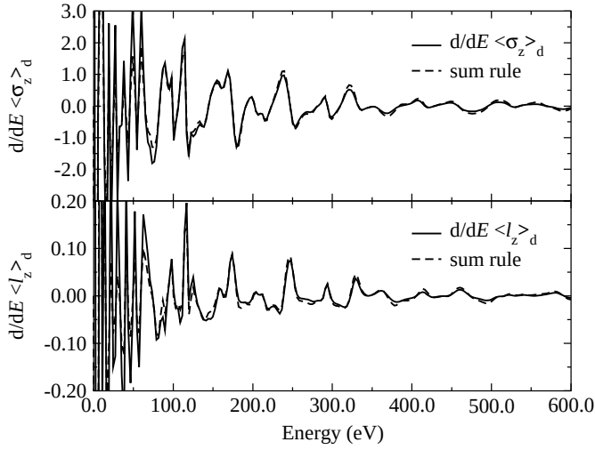
Fig. 7. Orbital polarisation \frac{d}{dE}\langle l_z \rangle_d (solid line) for the d-states of Pt in Fe 3 Pt compared to that derived from the MCXD spectra at the L 2,3 -edges (dashed line) using the differential sum rule in (31) (bottom). The upper panel gives the corresponding curves for the spin polarisation \frac{d}{dE}\langle \sigma_z \rangle_d . The small contribution \frac{d}{dE}\langle T_z \rangle_d has been ignored
