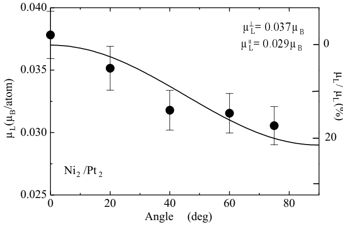
Fig. 11. Anisotropy of the orbital moment \mu_L for \text{Ni}_2/\text{Pt}_2 -multilayers determined from XMCD [44]. Although the absolute value of \mu_L is small its relative change is dramatically large, namely 22 %.
